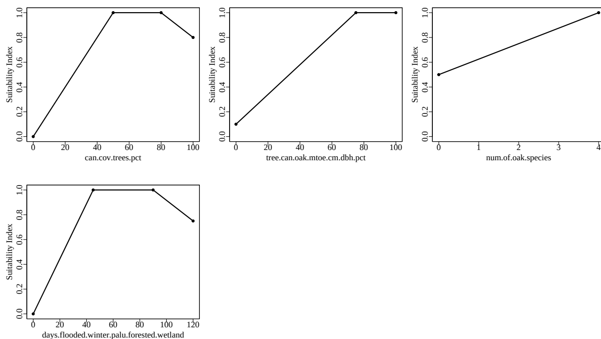
Figure 1. Suitability index graphs for variables included in the mallardForest-edPaluWetlands model in ecorest .
